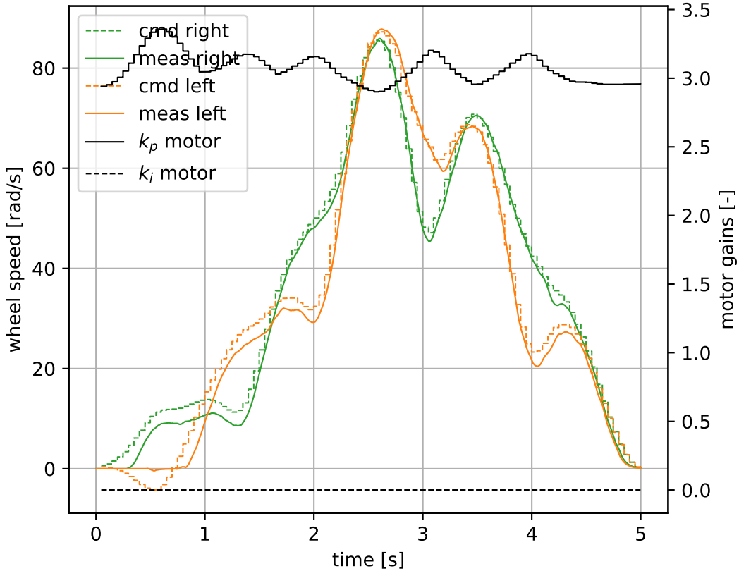
Wheel Speeds
